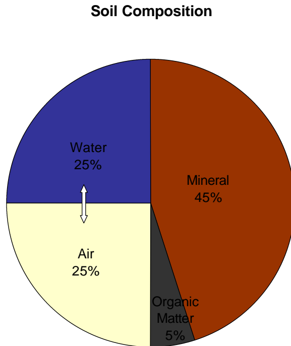
Figure 1. The relative proportion of mineral, organic matter, air and water in a soil that is optimum for growing plants.
